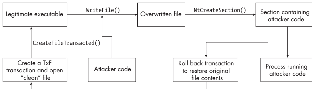
Figure 3-10: The execution flow of process doppelgänger
