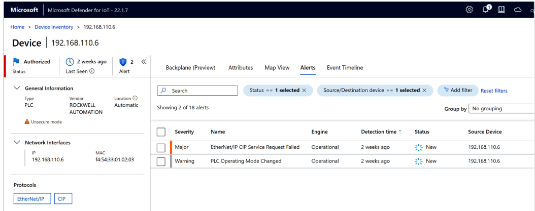
Figure 7.7 – Viewing the alerts on a device from the device inventory
