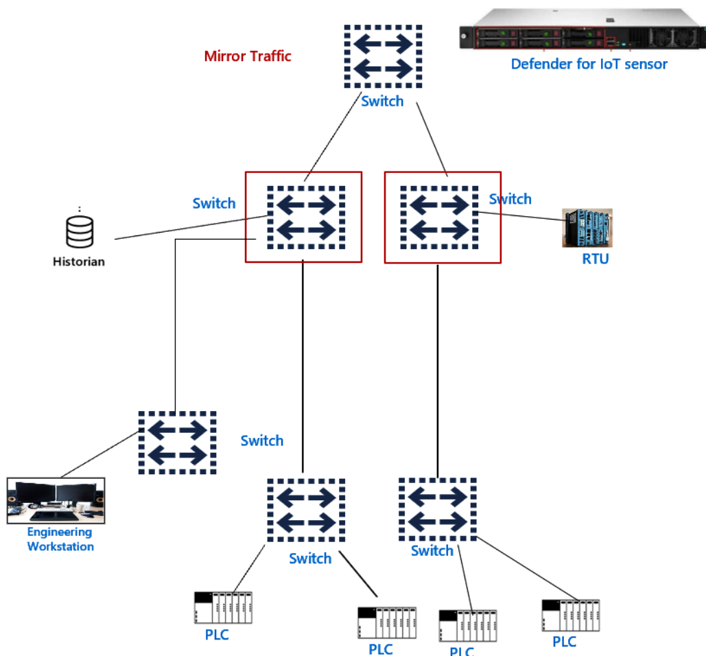
Figure 5.2 – The placement of an MDIoT sensor in a star topology
