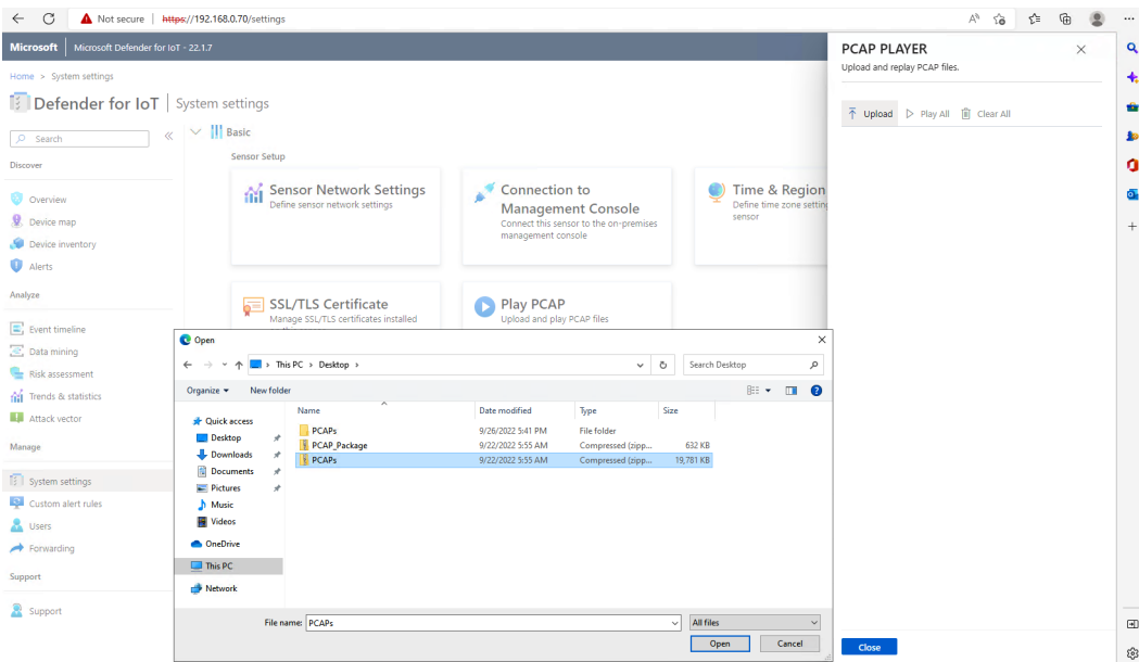
Figure 6.30 – Uploading PCAP files
