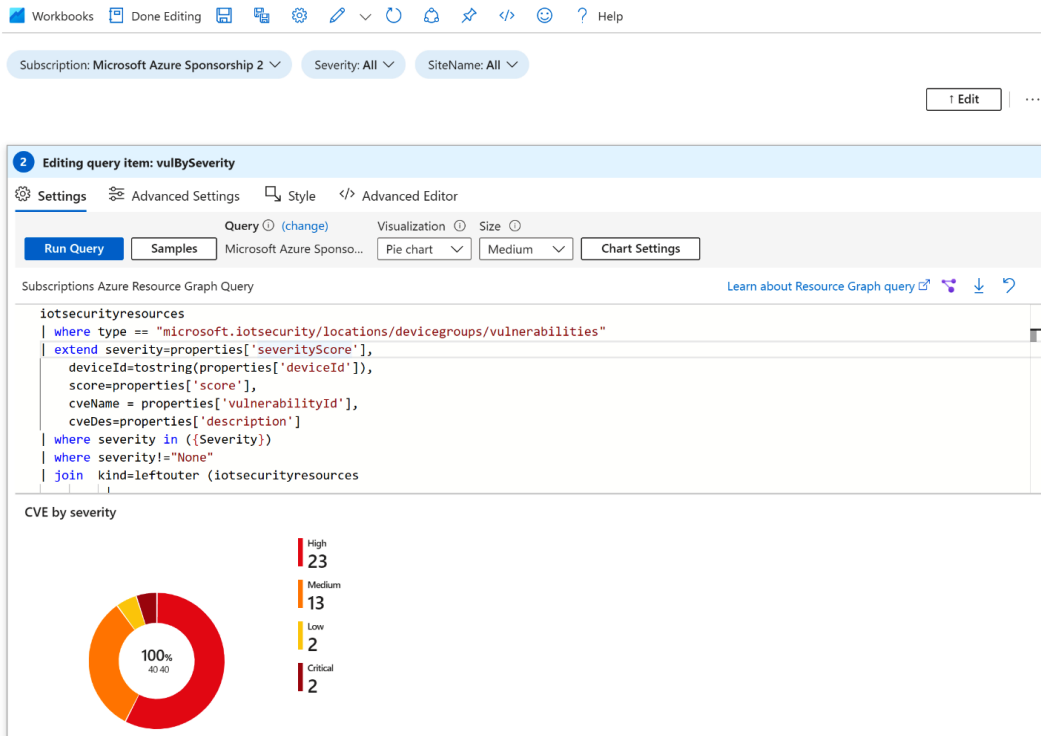
Figure 9.14 – The Vulnerabilities workbook – editing the dashboard
