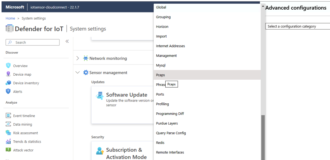
Figure 6.28 – Advanced configuration in the sensor console
