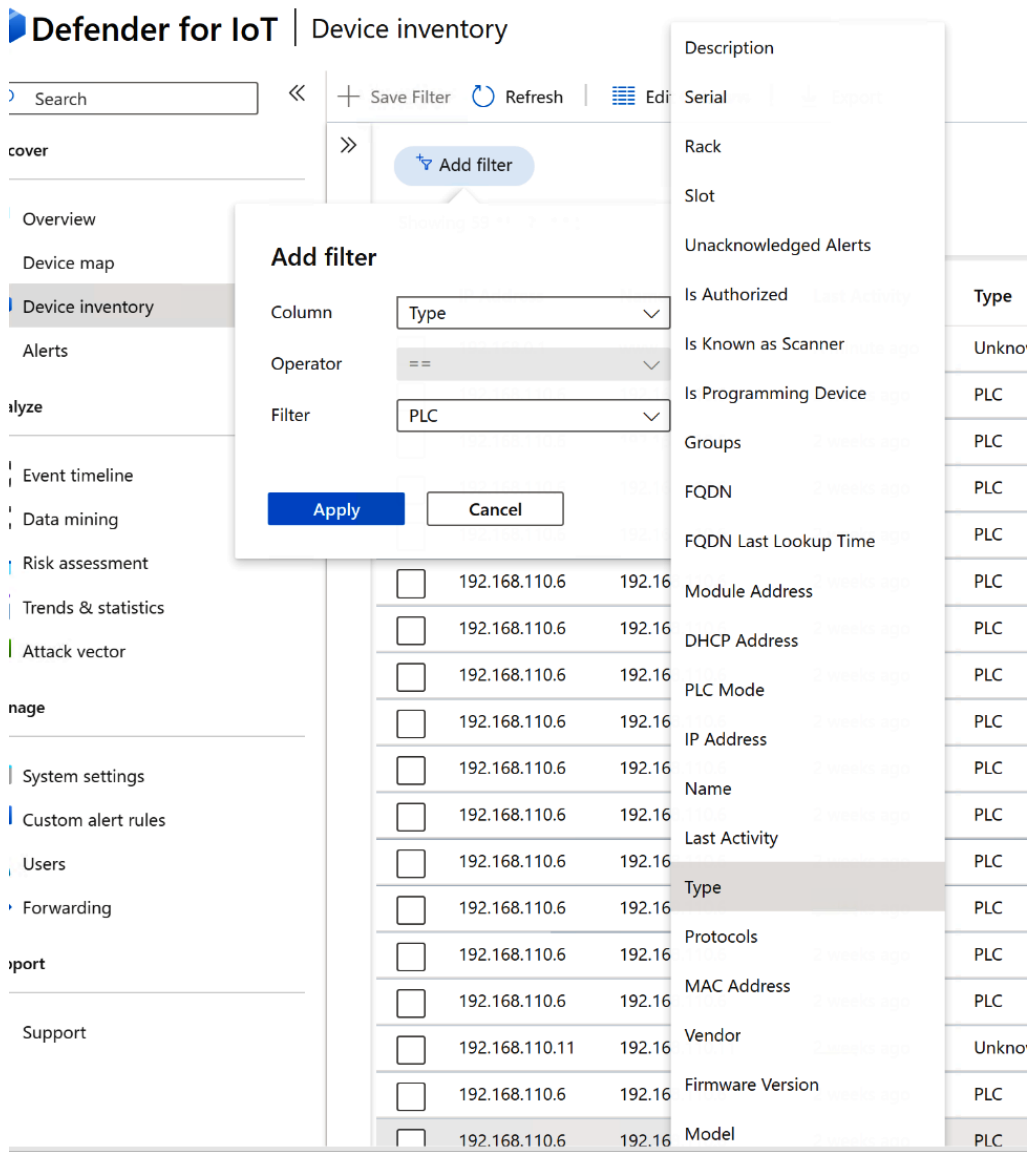
Figure 7.4 – Add filter in the device inventory
